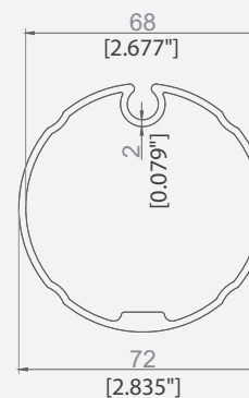
TUB 70 MM
