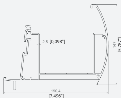
PROFIL JGHEAB OVAL 190,4X147
