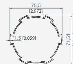
TUB MOTOR
